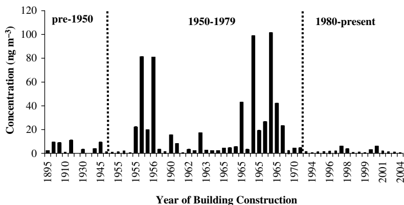
Figure 7.1 Variation of concentrations of \Sigma PCB in indoor air with date of building construction. (Reprinted with permission from Environmental Science and Technology, Causes of Variability in Concentrations of Polychlorinated Biphenyls and Polybrominated Diphenyl Ethers in Indoor Air , by Hazrati, S., Harrad, S., 40 (24), 7584–7589. Copyright (2006) American Chemical Society)
