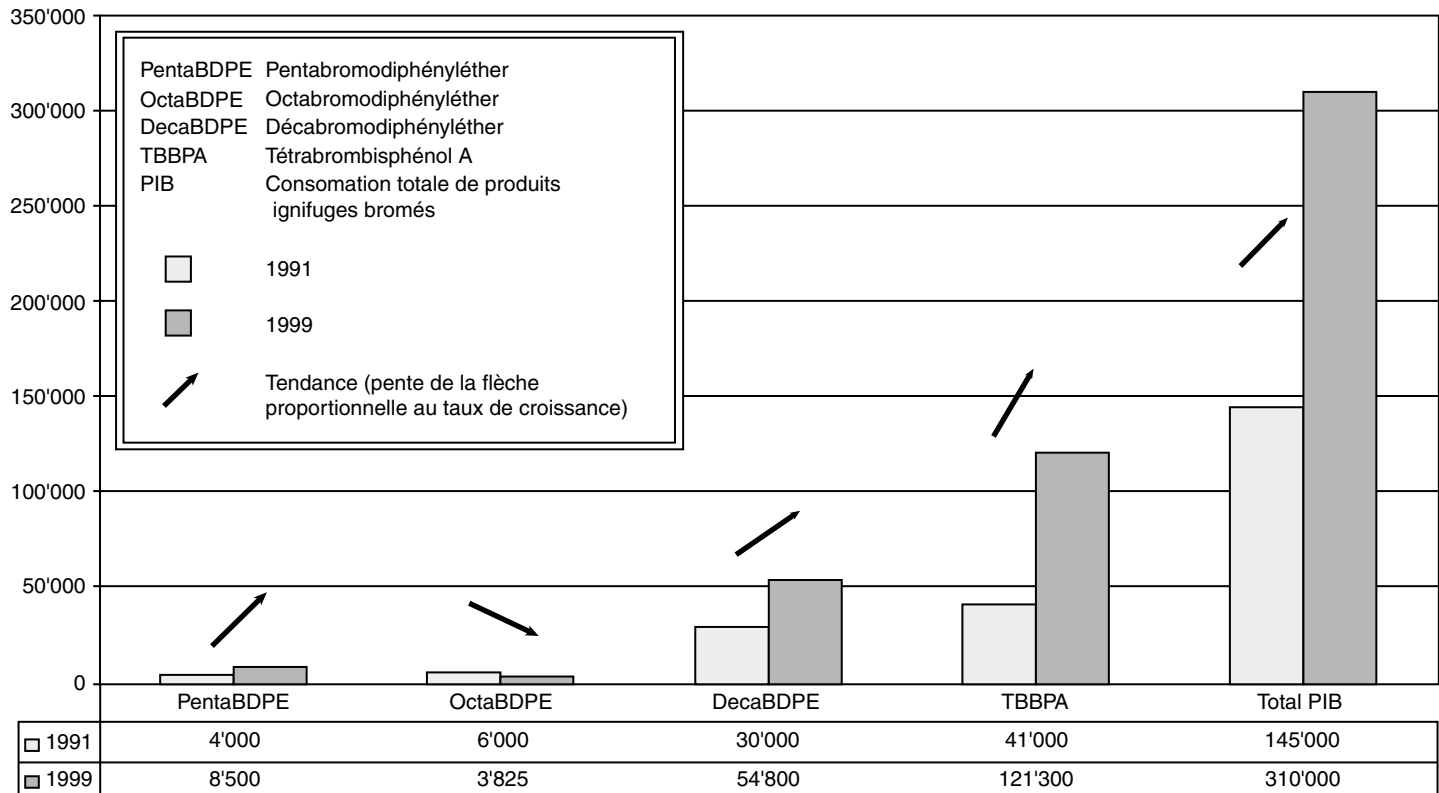
Figure 8.7 Consumption of BFRs in Switzerland estimated by Morf et al. 2003. (Reproduced with permission from Morf et al.)
