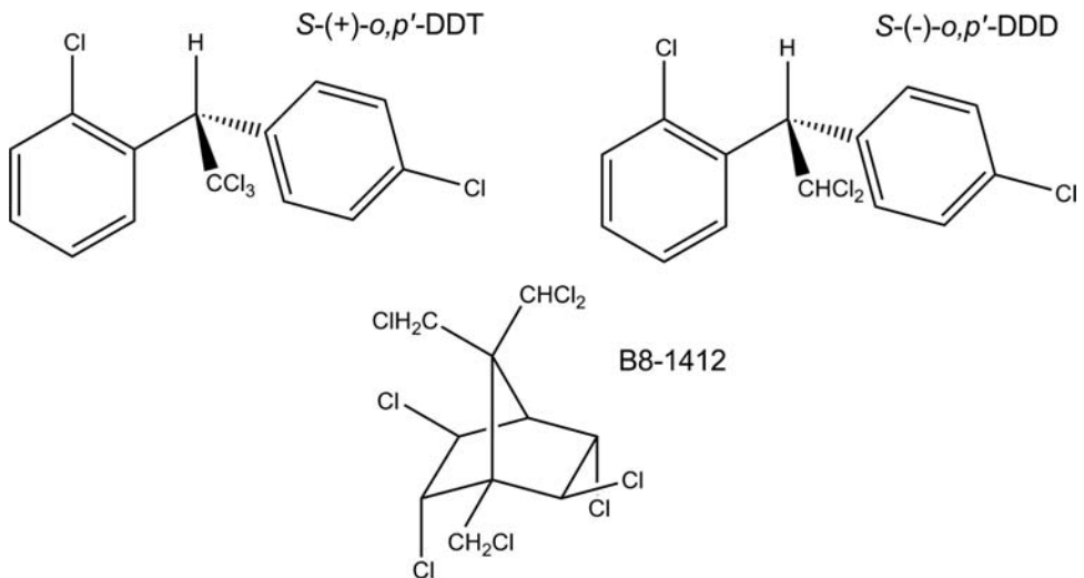
Figure 4.1 Structures of o,p' -DDT, o,p' -DDD, and toxaphene congener B8-1412 [256]. Only one enantiomer of each compound is depicted. Absolute configuration of chiral DDT components from Reference [31]
