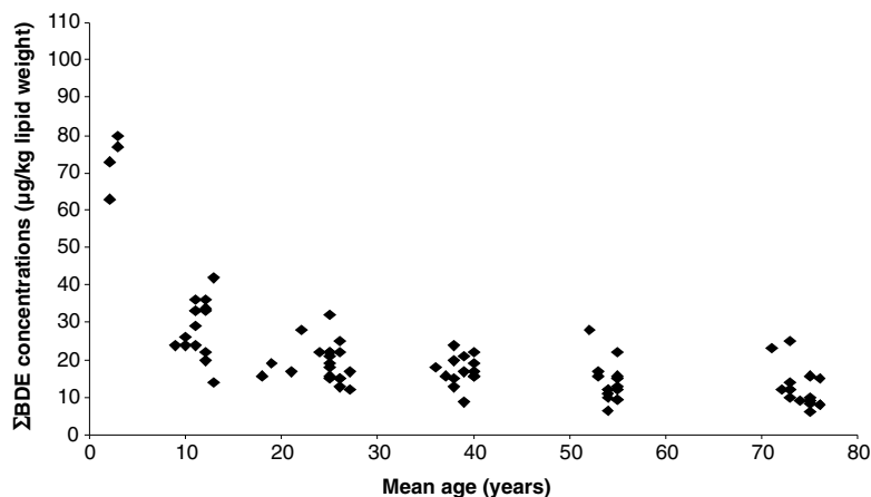
Figure 2.4 Summed BDE congener concentrations ( \mu\text{g}/\text{kg} lipid weight) in each pool of blood serum analysed by the respective mean age (in years) of donors in each pool. Each data point represents a pool of up to 100 blood samples. (Reproduced by permission from Environmental Science and Technology, Higher Accumulation of Polybrominated Diphenyl Ethers in Infants Than in Adults , by Toms, L.-M. L., Harden, F., Paepke, O., Ryan, J. J., Hobson, P., Mueller, J. F., 42 (19), 2510–2515. Copyright 2008 American Chemical Society)
